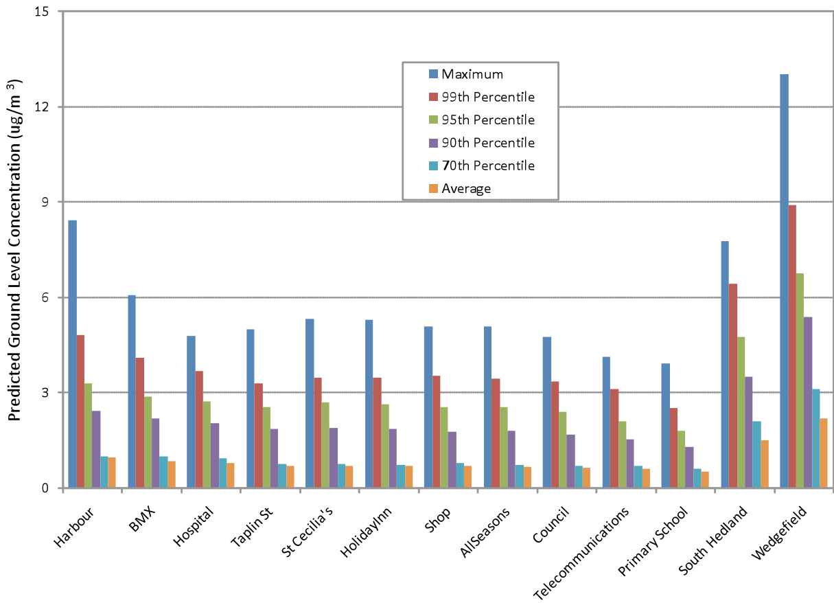
Figure 8.5 – Statistics of Predicted 24-hour PM 10 Ground Level Concentrations from the Proposed Outer Harbour Development (standalone with no background)
