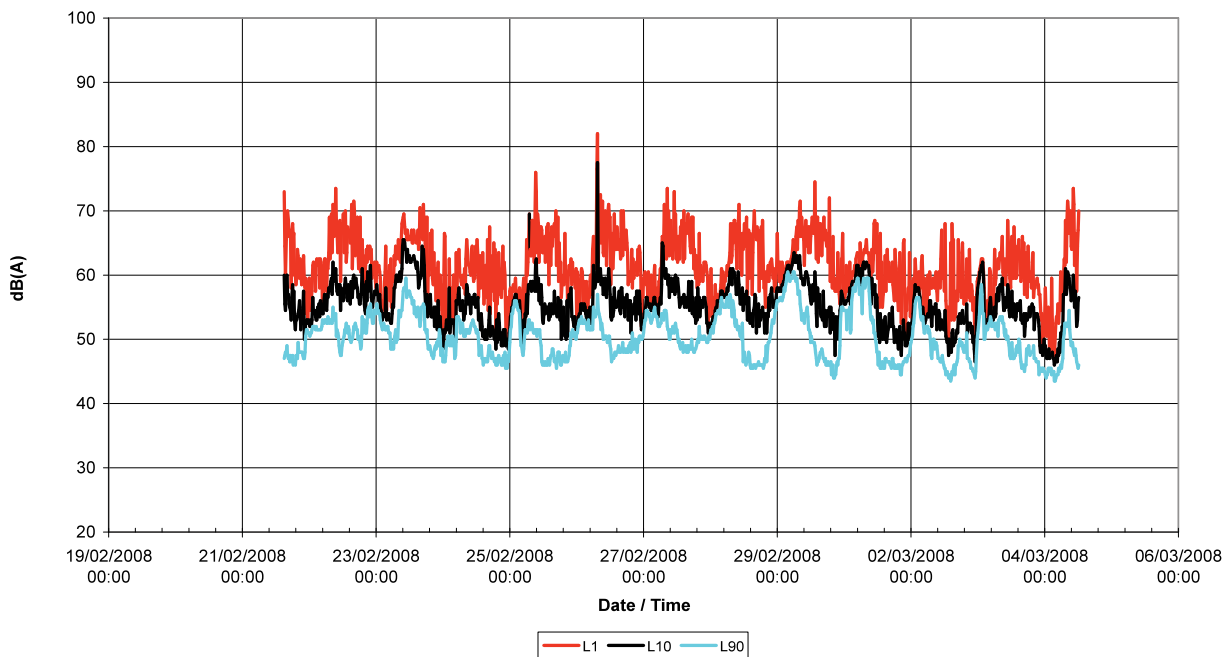
Figure 8.7 – Ambient Noise Levels Recorded at the Hospital Site, Port Hedland 22 February to 5 March 2008
